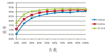
RSD-150D-12
