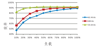
RSD-150C-24
