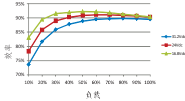
RSD-150C-12
