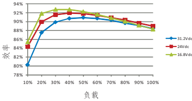
RSD-150C-5
