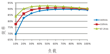
RSD-150D-5
