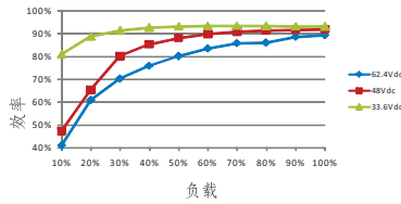
RSD-150C-12
